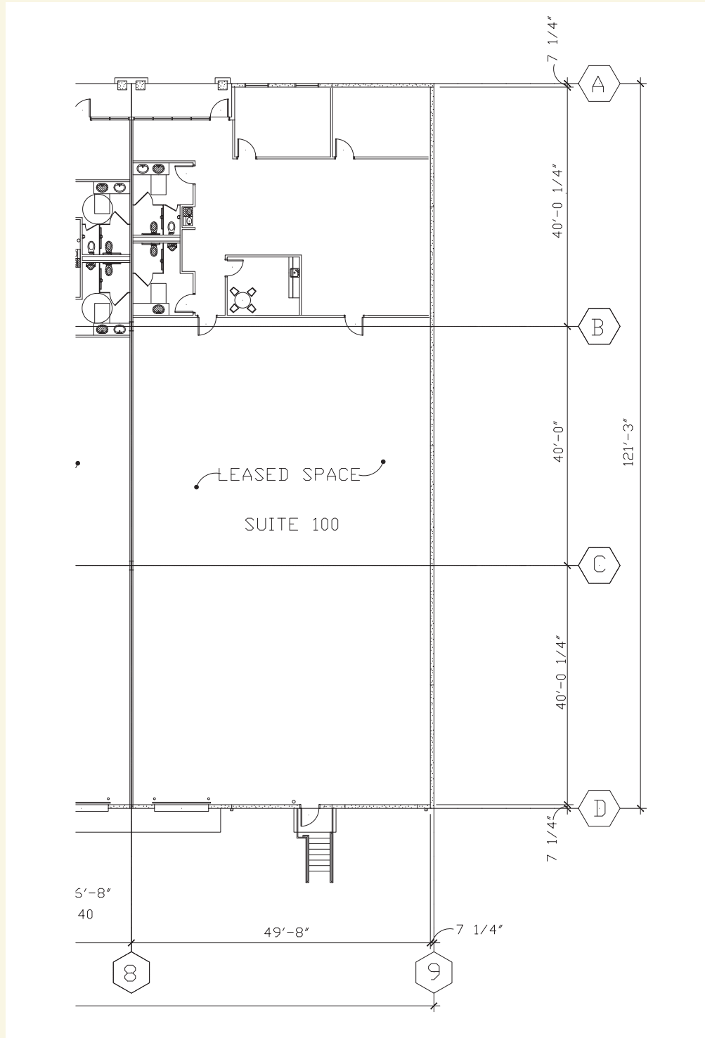
SUITE 100 FLOOR PLAN
